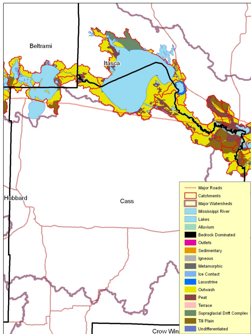
Figure 3. Surficial Geology
