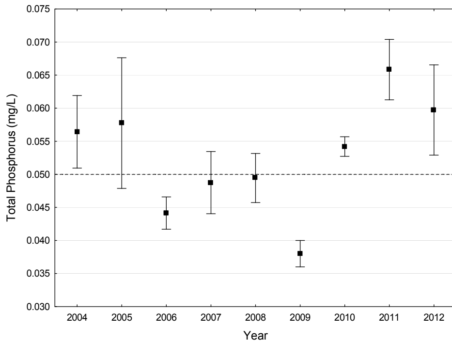
Figure 105. Growing season (June-Sept) mean \pm SE total phosphorus concentration per year on 07010104-503. The dotted line indicates the proposed water quality standard (0.05 mg/L).
