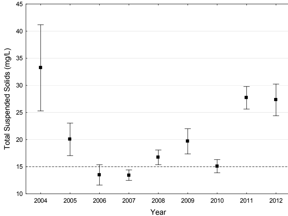
Figure 107. Growing season (Apr-Sept) mean \pm SE total suspended solids concentration per year on 07010104-503. The dotted line indicates the water quality standard (15 mg/L).
