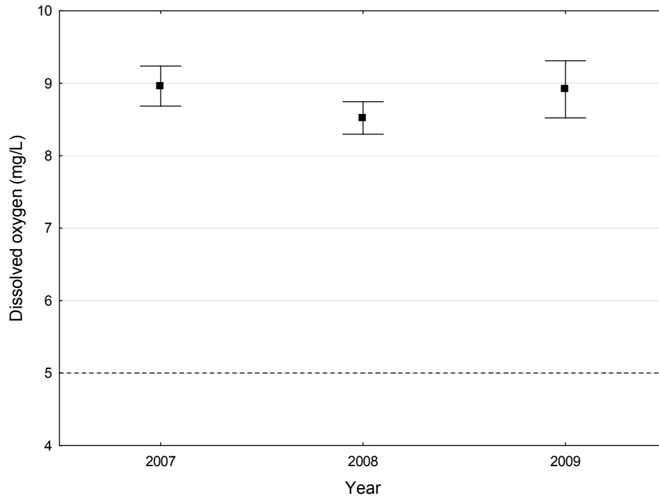
Figure 96. Mean \pm SE dissolved oxygen concentration per year on 07010103-505. The dotted line indicates the water quality standard for dissolved oxygen ( >5.0 mg/L).
