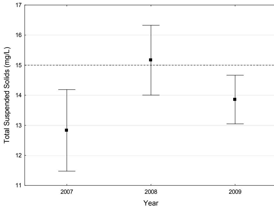
Figure 97. Growing season (Apr-Sept) mean \pm SE total suspended solids concentration per year on 07010103-505. The dotted line indicates the water quality standard (15 mg/L).
