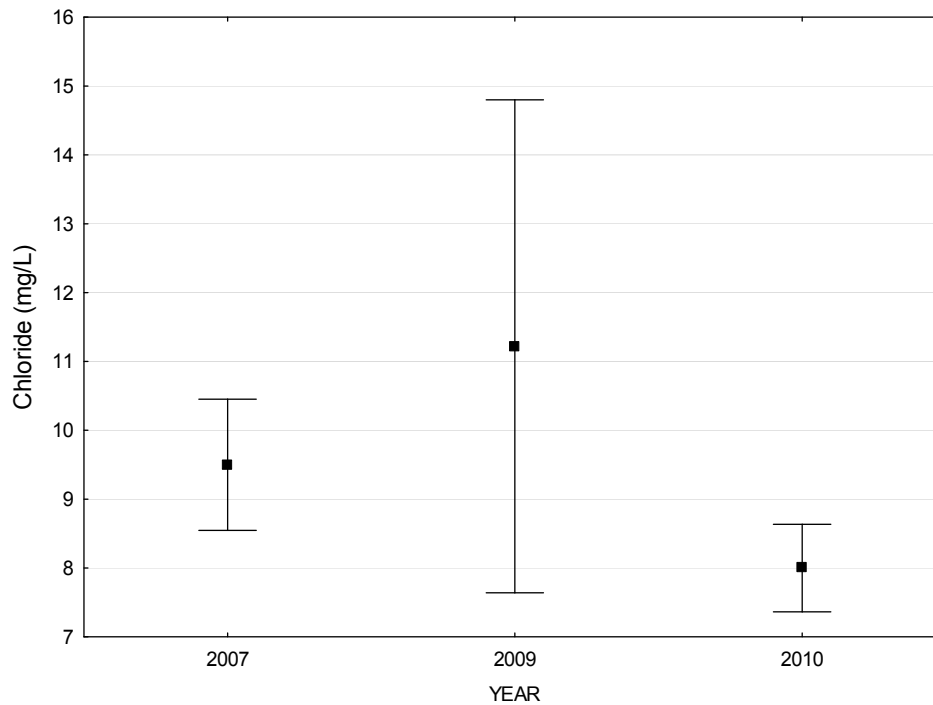
Figure 117. Mean \pm SE chloride concentration per year on 07010104-577. The water quality standard for chloride is 230 mg/L.
