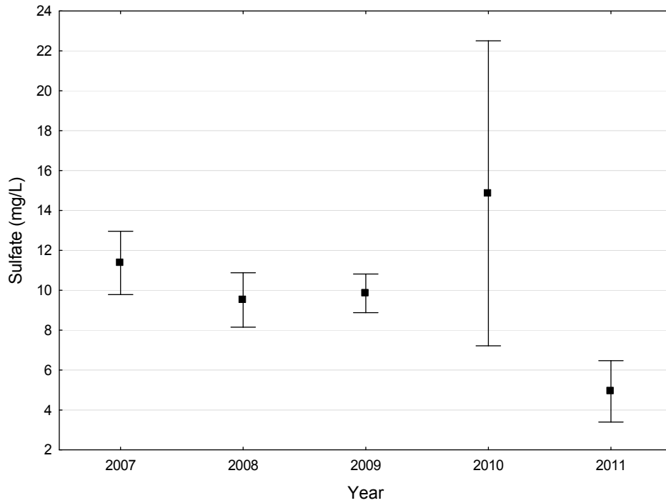
Figure 132. Mean \pm SE sulfate concentration per year on 07010201-501. The water quality standard for sulfate is 250 mg/L.
