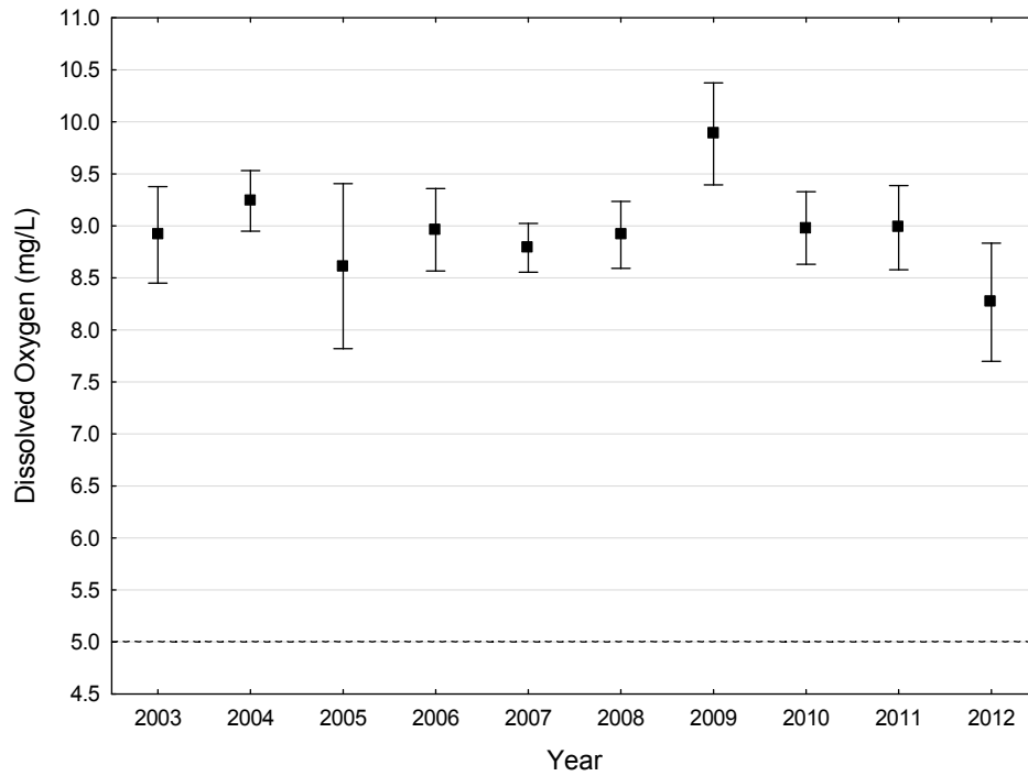
Figure 102. Mean \pm SE dissolved oxygen concentration per year on 07010104-503. The dotted line indicates the water quality standard for dissolved oxygen (>5.0 mg/L).
