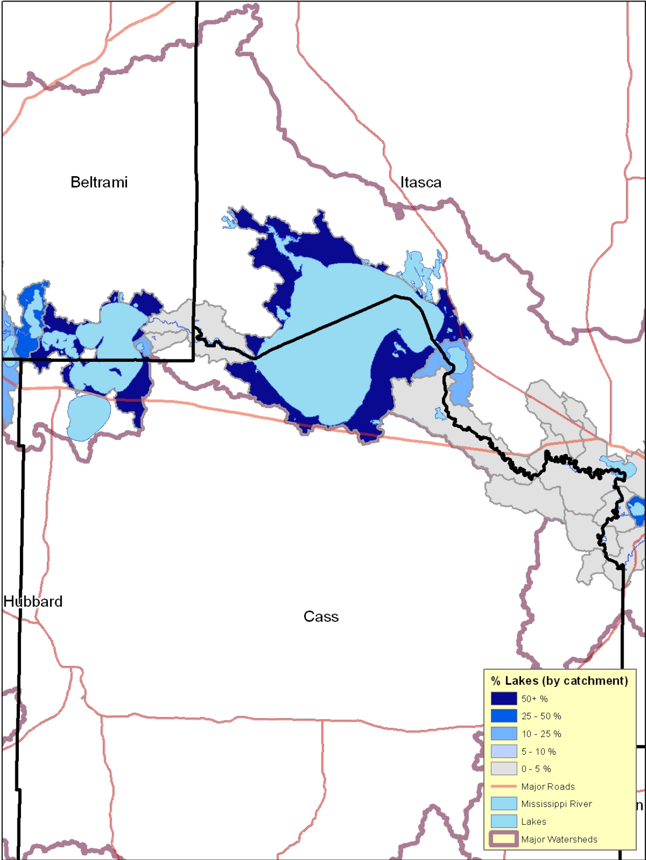
Figure 10. % Lakes
