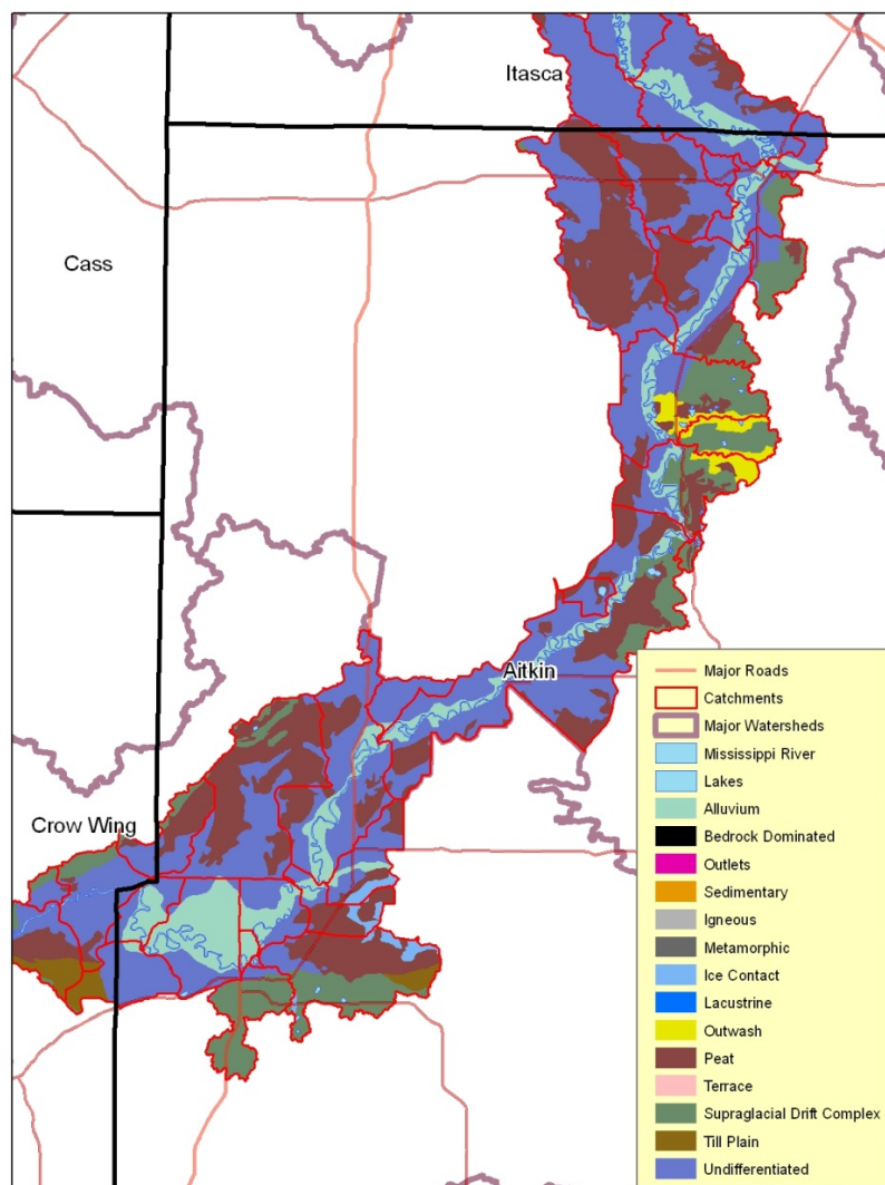
Figure 3. Surficial Geology
